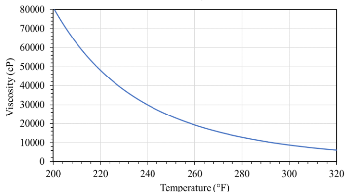
Uncured Viscosity Curve
